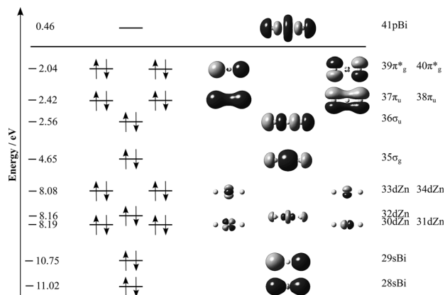
Figure 3. Molecular orbital diagram for the linear [\text{Bi–Zn–Bi}]^{4-} unit calculated at the BP/SVP/PCM level (acetonitrile, \epsilon = 36.64 ) [26] .
